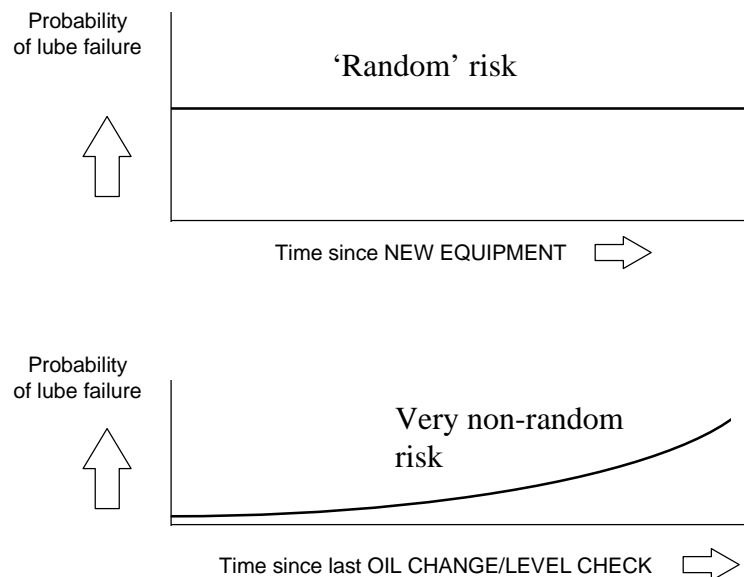
Figure 4. 'Random' is relative: lubrication failures example
